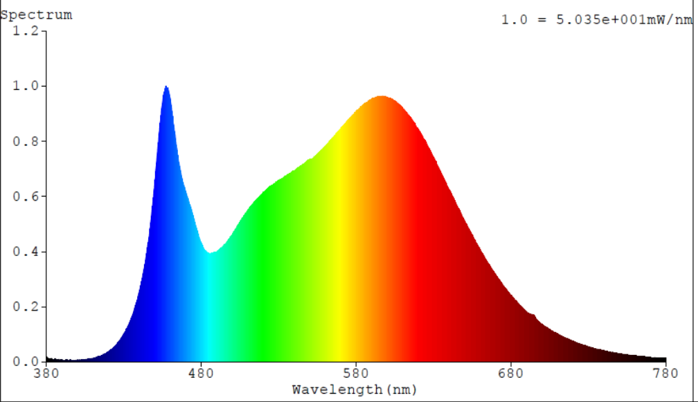
Spectral Distribution
