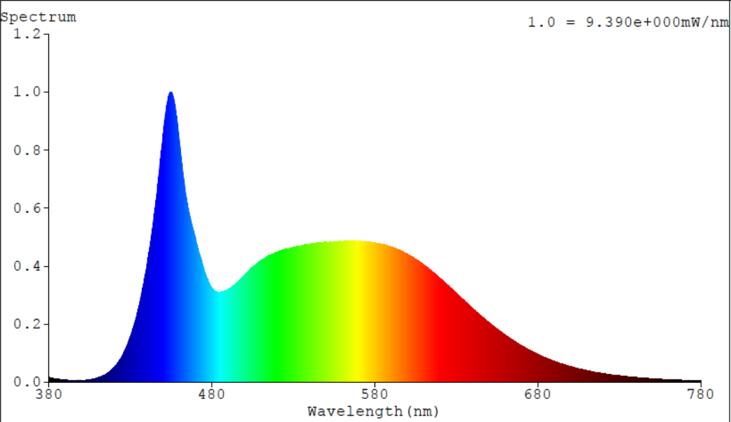
Spectral Distribution
